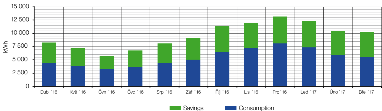
Monthly consumption and energy savings graph in a system with LED luminaire voltage regulation
